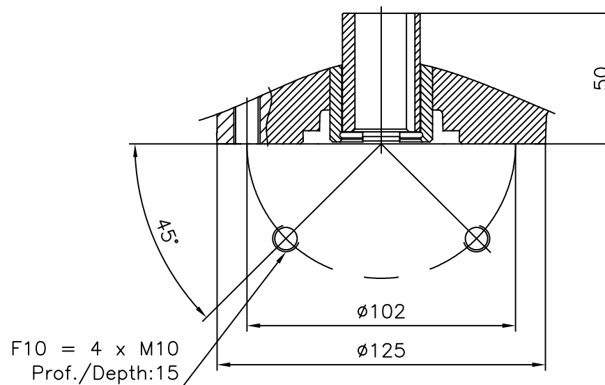
ISO 5210 Vue A de la bride View A of the flange Echelle/Scale: 1/2
