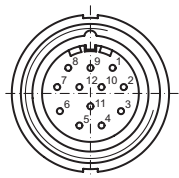
Connector M23, female, 12-pin, clockwise (CW)
