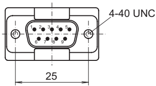
Connector D-SUB, pin contacts, 9-pin
