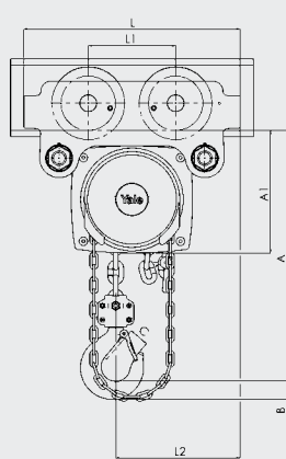
YALELIFT ITP ATEX, SINGLE FALL 1/4 TO 2-TON
