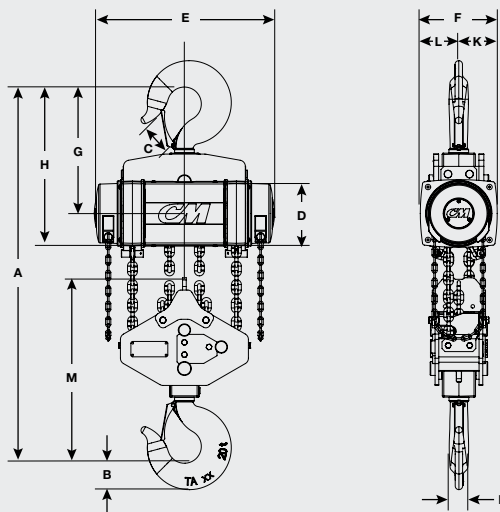
HOOK-MOUNTED HOIST 15 & 20-TON
