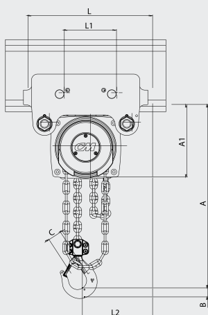
YALELIFT 360° ATEX, SINGLE FALL 1/4 TO 2-TON
