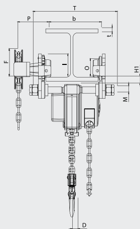
YALELIFT 360° ATEX, SINGLE FALL 1/4 TO 2-TON
