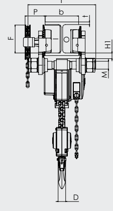
GEARED TROLLEY HOIST 5-TON
