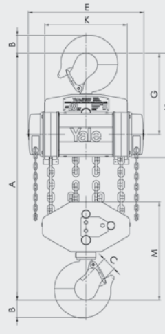
YALELIFT 360° ATEX, SIX FALL 8 TO 12-TON
