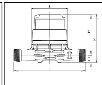
DN20 composite
