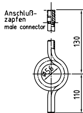
Kreisform (FORM D)
