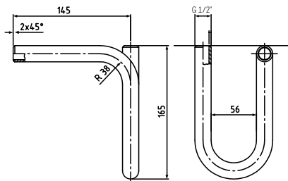
U-Form (FORM B)
