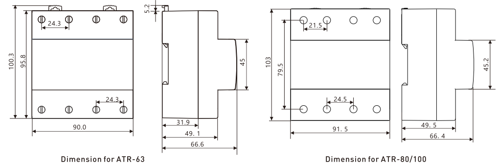
Dimension for ATR-63
