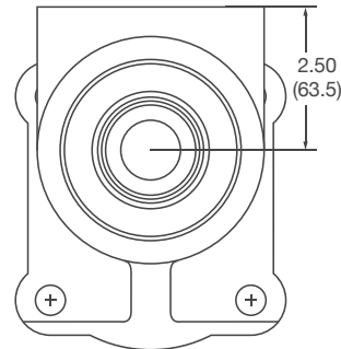
Pad Mount
