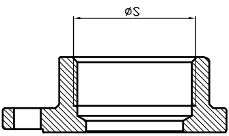
SOCKET WELD TYPE
