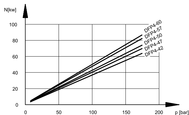
ABSORBED POWER/PRESSURE CURVES (measured at 1500 rpm)
