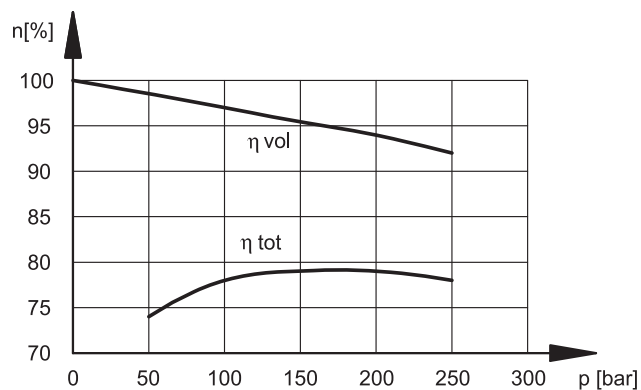
VOLUMETRIC AND TOTAL EFFICIENCY
