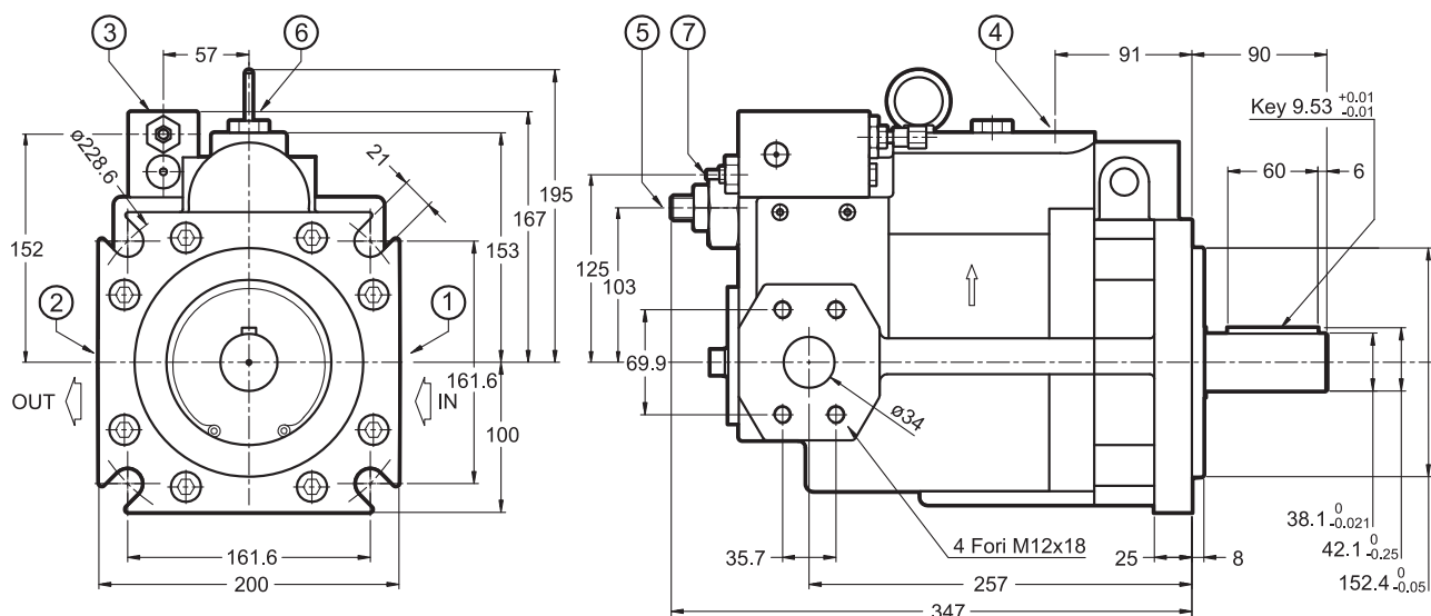
VPPL-100PC6 PUMP
