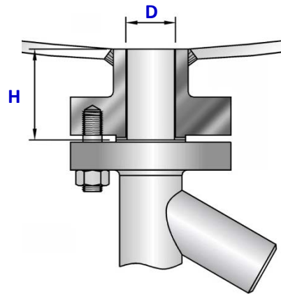
Nozzle
