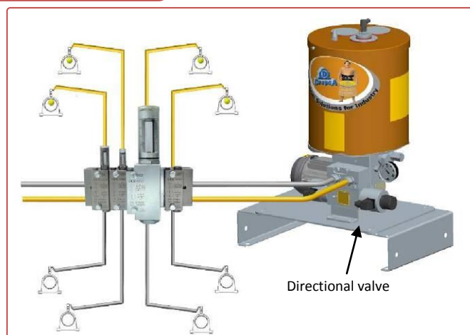
PRESSURE LINE 2
