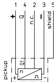
connection diagram
