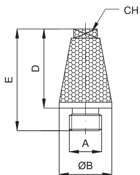
Truncated cone with wrench in top
