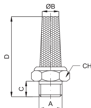
Extended truncated cone with hex. key on nipple
