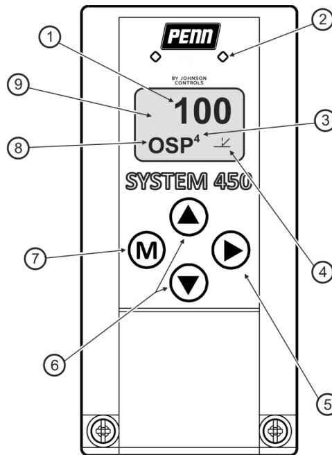
Figure 1: System 450 control module output analog LEDs, LCD, four-button touchpad UI
