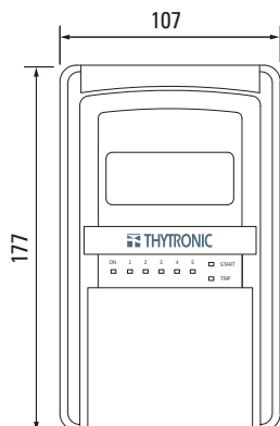
FLUSH MOUNTING
