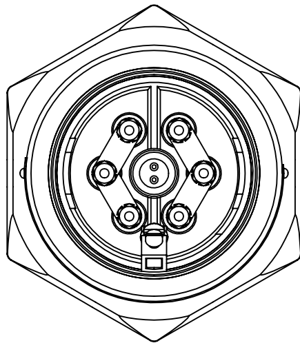
1 PHASE PARALLEL W/T-STAT
