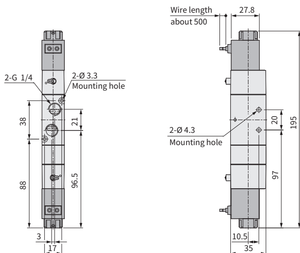
SX 6232 (Closed center) N.C.
