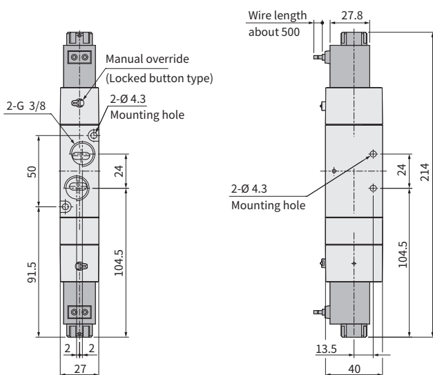
SX 8233 (Closed center) N.C.
