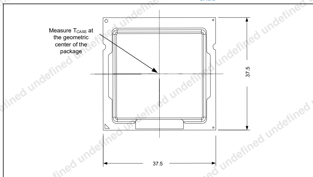
Figure 5-6. Thermal Test Vehicle (TTV) Case Temperature ( T_{\text{CASE}} ) Measurement Location
