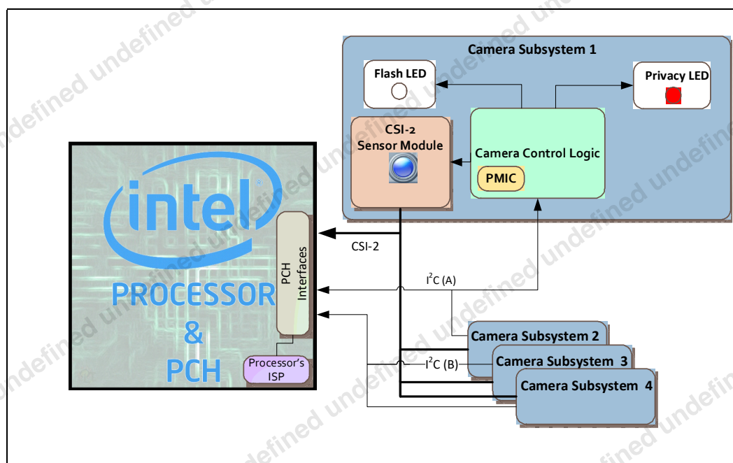
Figure 3-2. Processor Camera System
