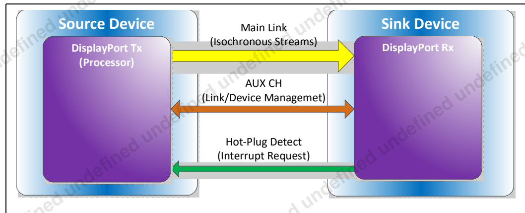
Figure 2-7. DisplayPort* Overview
