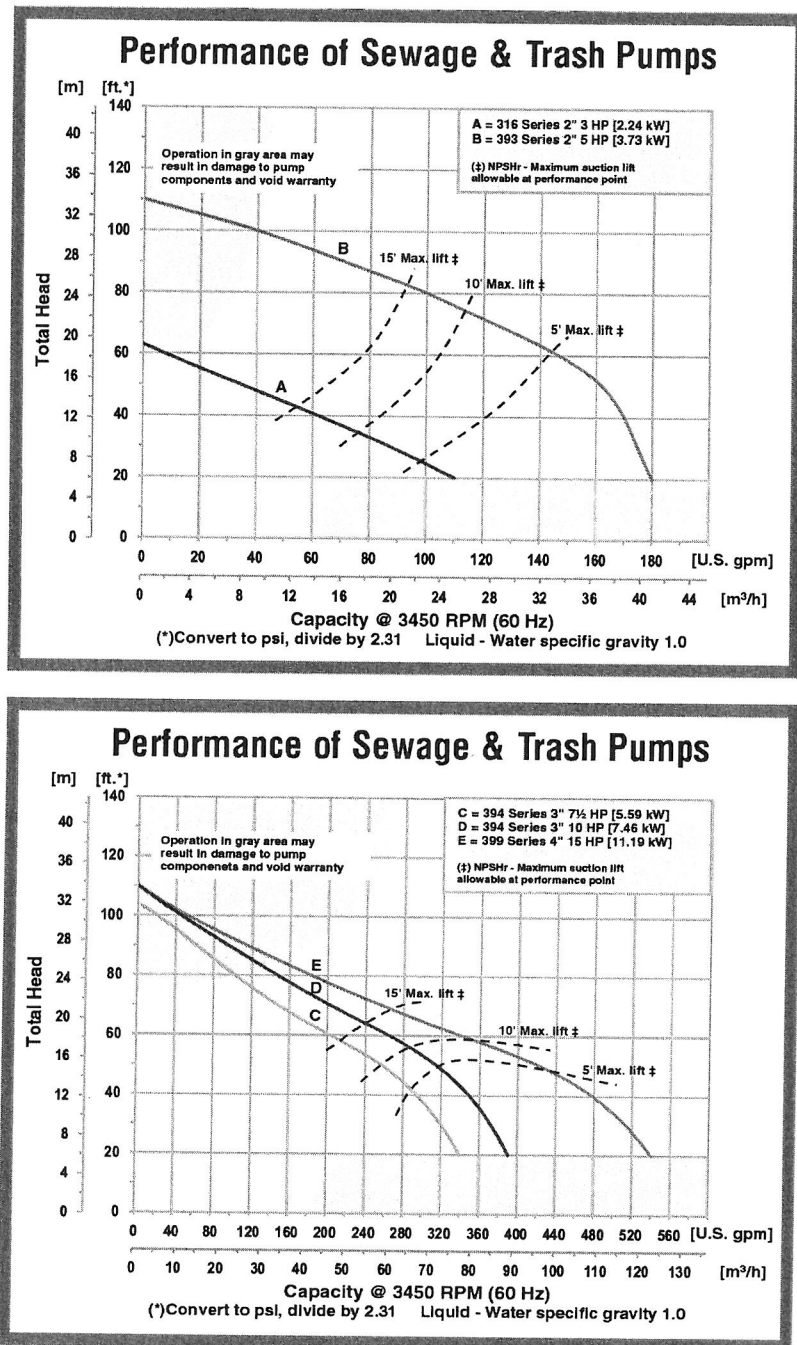
Figure 3 - Performance Curve
