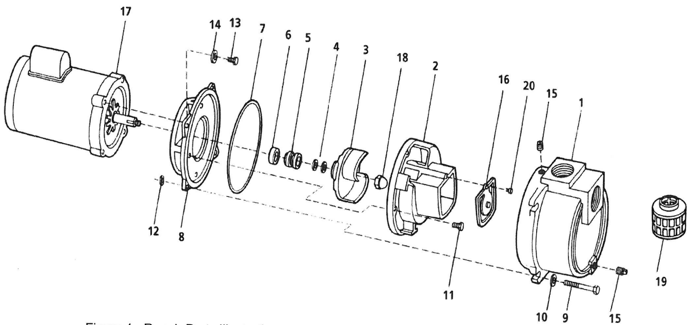
Figure 4 - Repair Parts Illustrations
