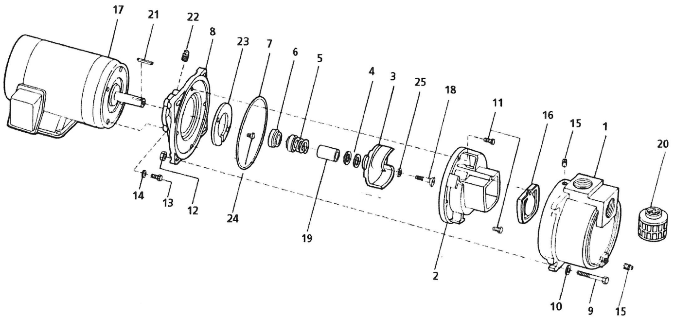
Figure 5 - Repair Parts Illustrations
