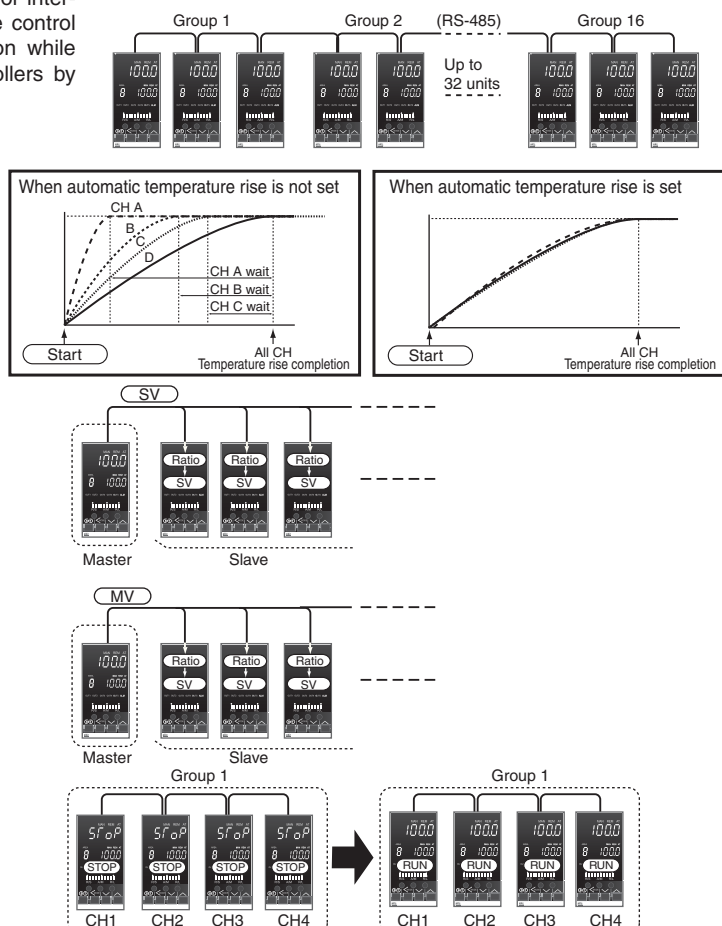
Inter-controller Communication
