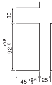
Panel Cutout
