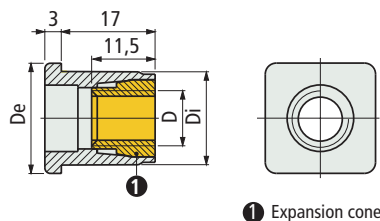
Tube dimensions
