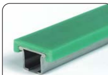
Part. S0367 - Pag. S24 Multiple strands 82,5 mm (K 325)/ pitch 85-83,5 mm.
