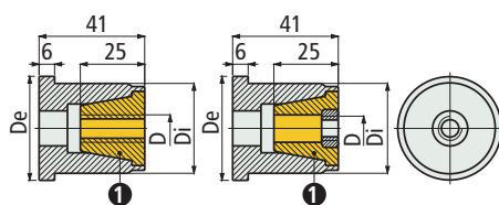
Tube dimensions
