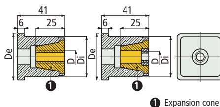
Tube dimensions
