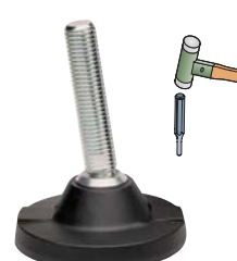
Part. R0297 - Pag. R27 Ø 124 • Prefitting for fixing • Max. load 45000 N.
