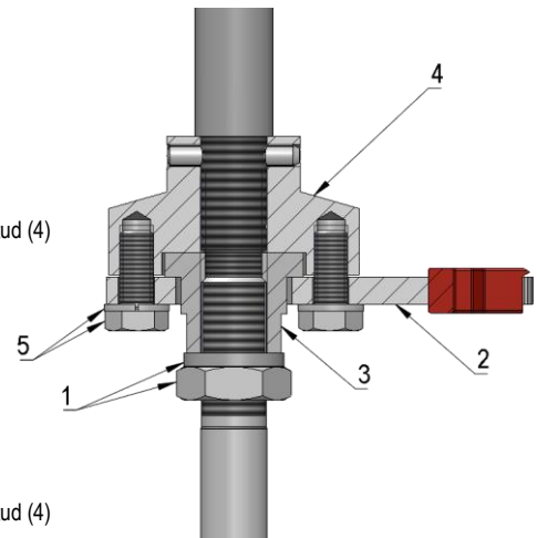
(5) 90° offset drawn
