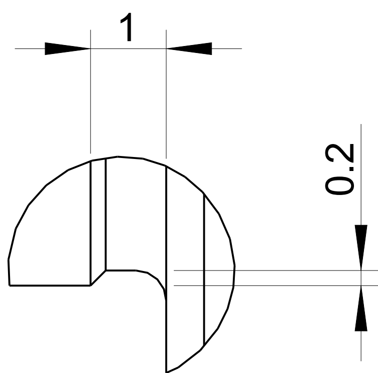
DETAIL A SCALE 20:1
