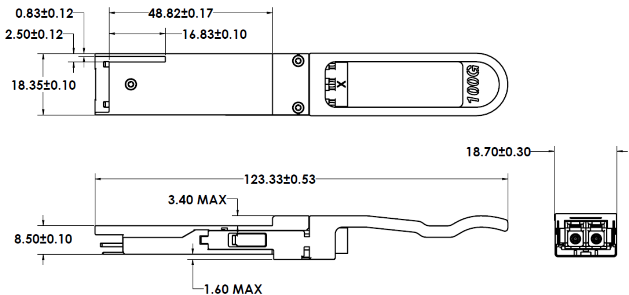
Figure 2. FTLC1156RDPL Mechanical Dimensions.
