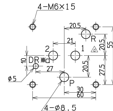
Mounting holes dimension
