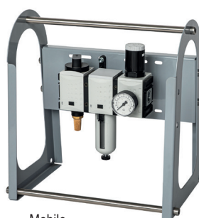
Mobile maintenance unit
