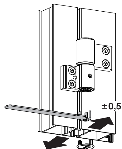
Compression adjustment
