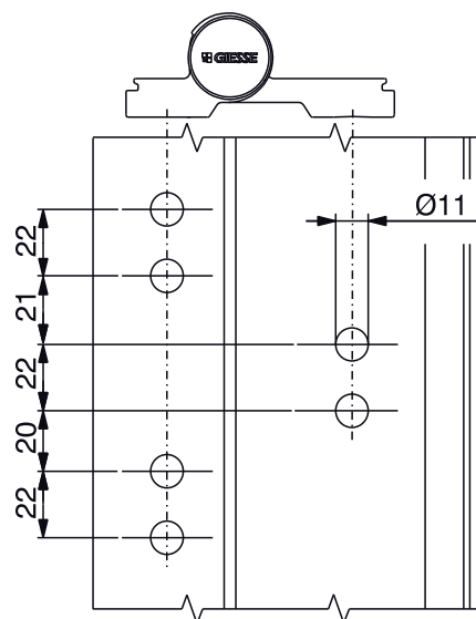
Machining on profile for three-wing hinge
