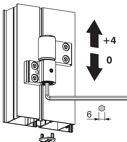
Height adjustment
