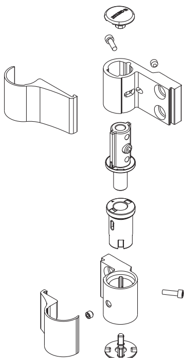
Height adjustment
