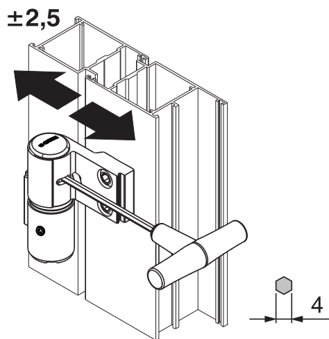
Side adjustment
