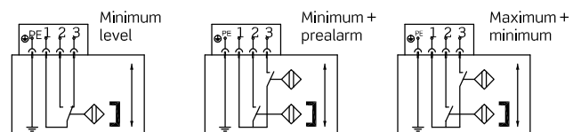
Level switch characteristics
