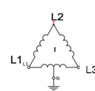
Three Phase Delta Hi Leg, 4 W + G
