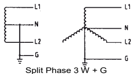
Split Phase 3 W + G
