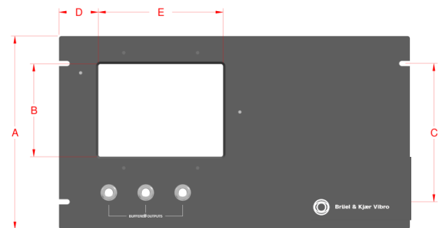
FACEPLATE
