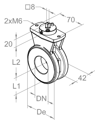
Square shaft
