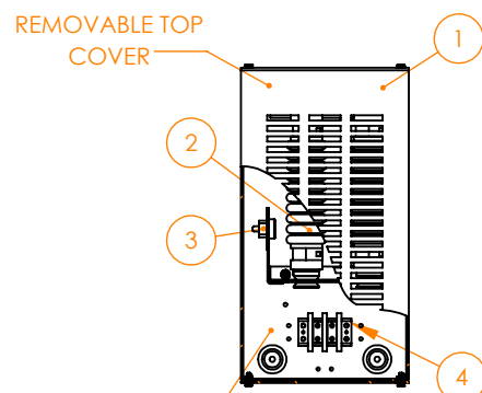
CABLE SPACE— TOP VIEW (BROKEN OUT SECTION)
