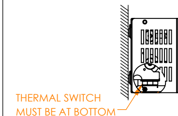
SIDE VIEW [R] (VERTICAL MOUNTING)
