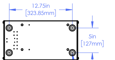
BOTTOM VIEW (MOUNTING DIMENSIONS)
