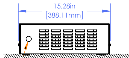
FRONT VIEW (HORIZONTAL MOUNTING)
