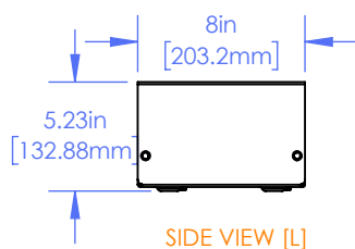
SIDE VIEW [L]
