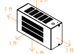
VERTICAL MOUNTING
