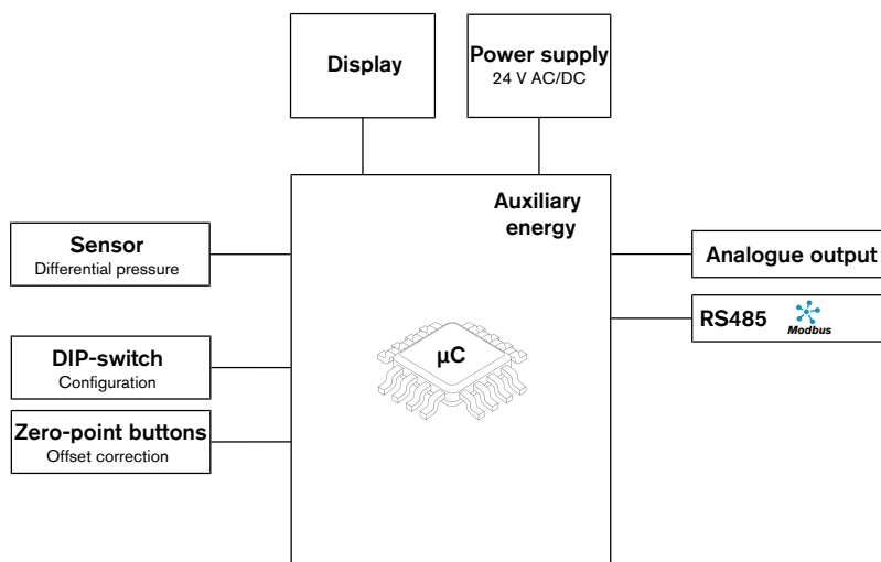
Fig. 1: Function diagram
