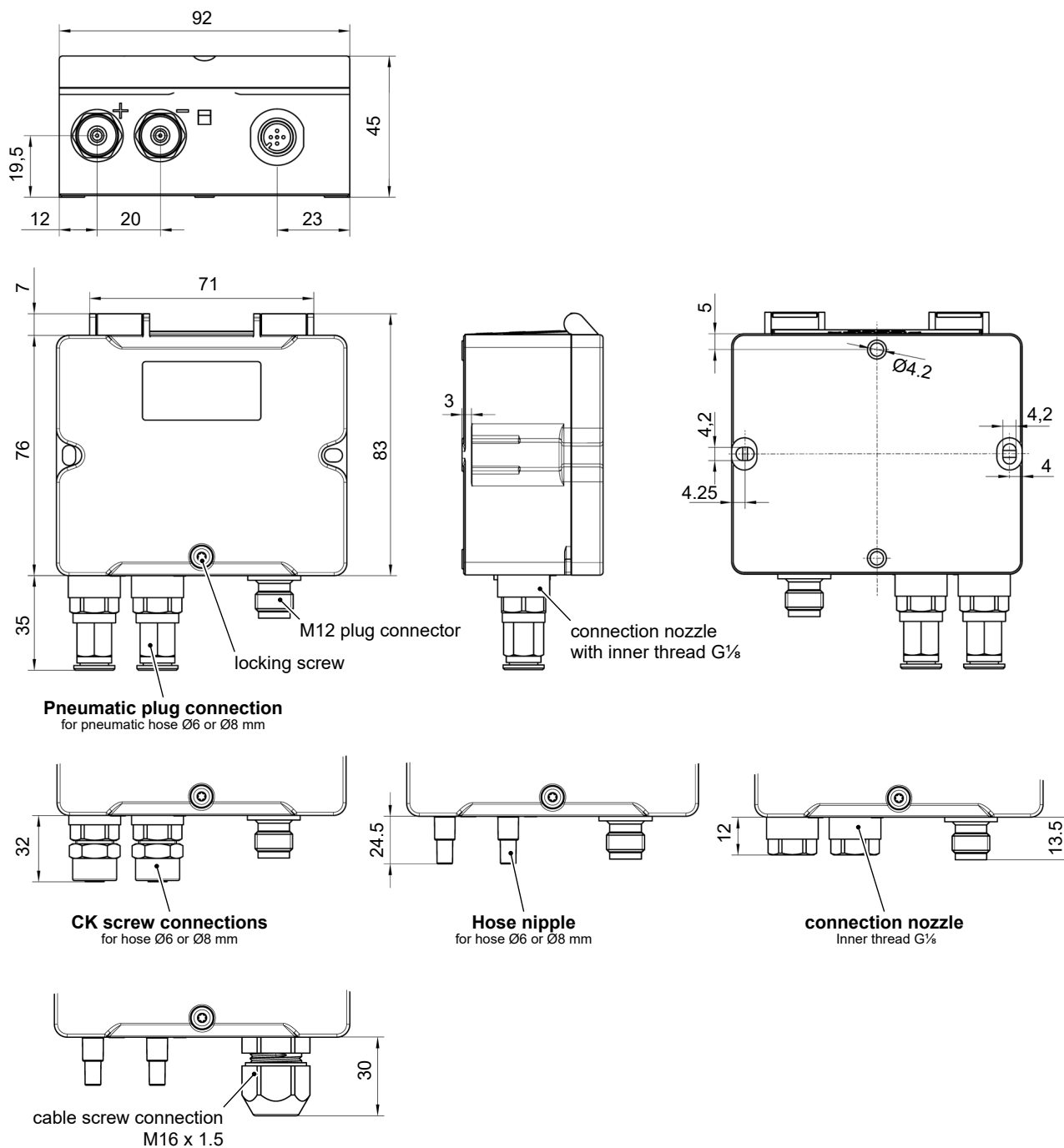
Fig. 4: Dimension drawing
