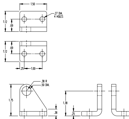
Trunnion Brackets
