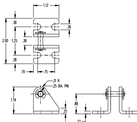
Pivot Bracket
