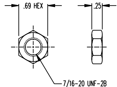
Mounting Nut
