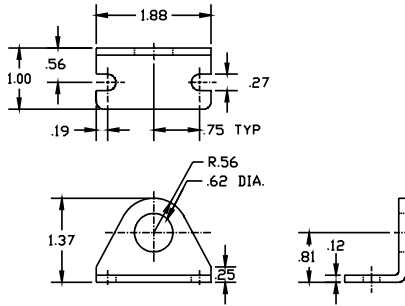
Foot Bracket
