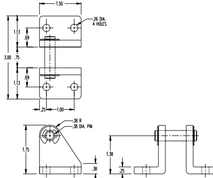
Pivot Brackets
