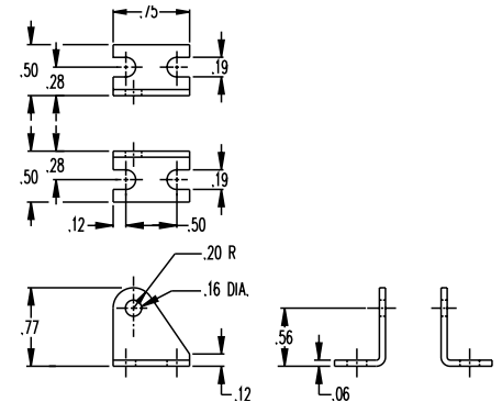
Pivot Brackets
