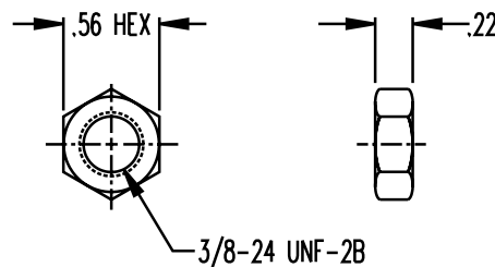
Mounting Nut
