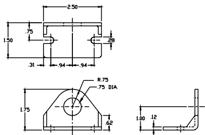
Foot Bracket
