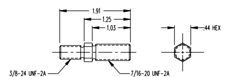
1-1/2" Bore D-6636
