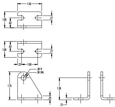
Pivot Bracket
