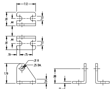
Pivot Brackets
