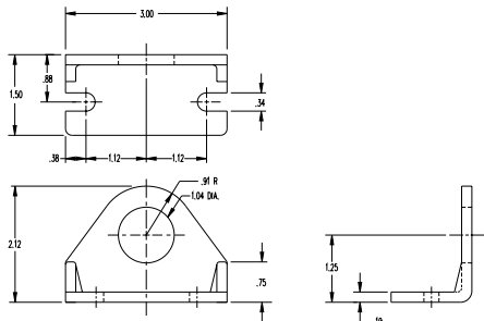
Mounting Bracket
