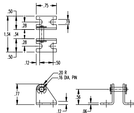
Pivot Bracket with Pin
