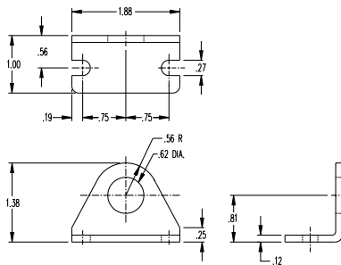
Mounting Bracket
