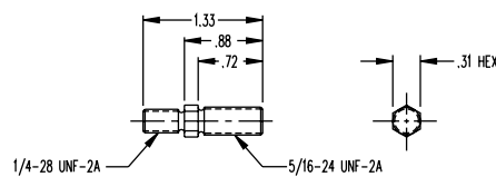
1-1/16" Bore D-6583
