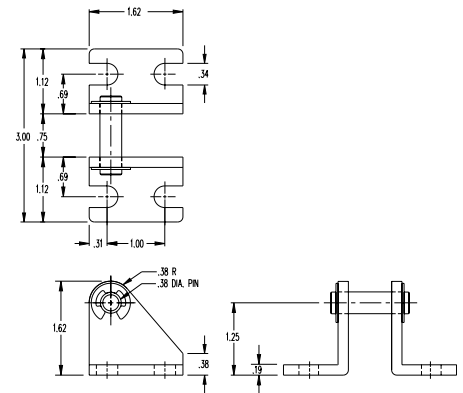
Pivot Bracket
