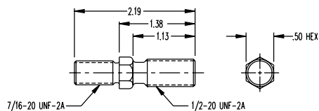
2" Bore D-6637
