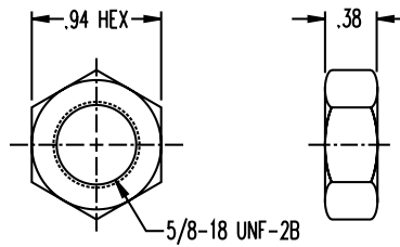
Mounting Nut
