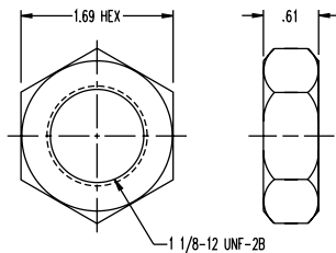
Mounting Nut
