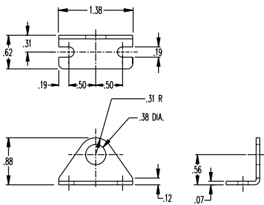
Mounting Bracket (for Single Acting Models)
