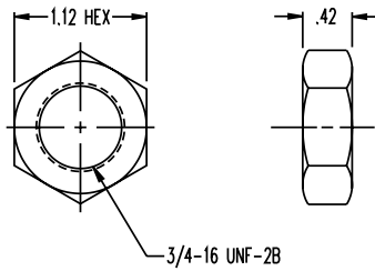
Mounting Nut
