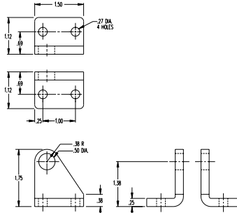
Trunnion Brackets
