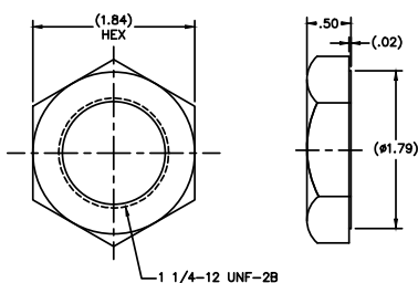
Mounting Nut
