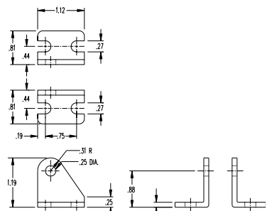
Pivot Brackets
