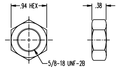
Mounting Nut
