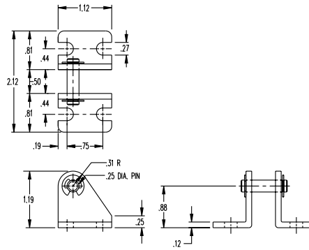
Pivot Brackets
