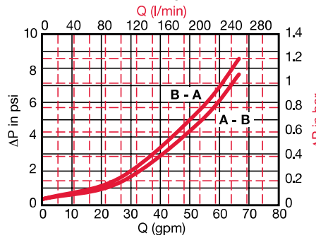
DFF 330/660/1320 Housing
