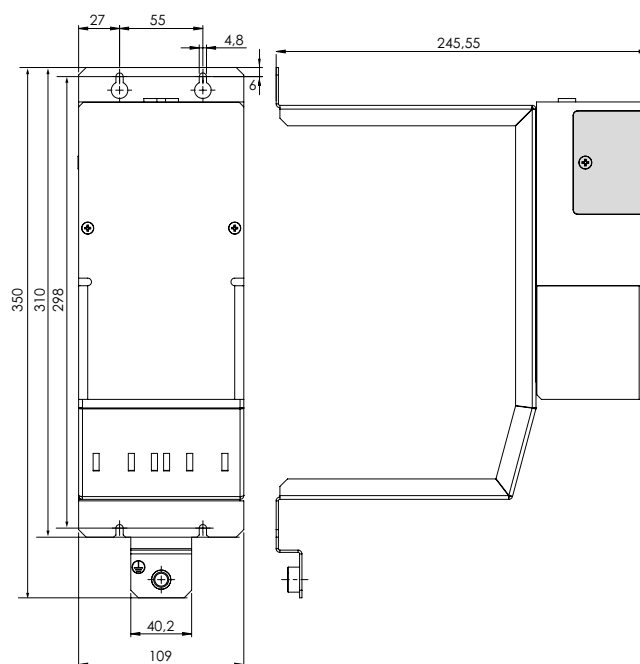
Figure 7.13 D3-XV 300/A dimensions
