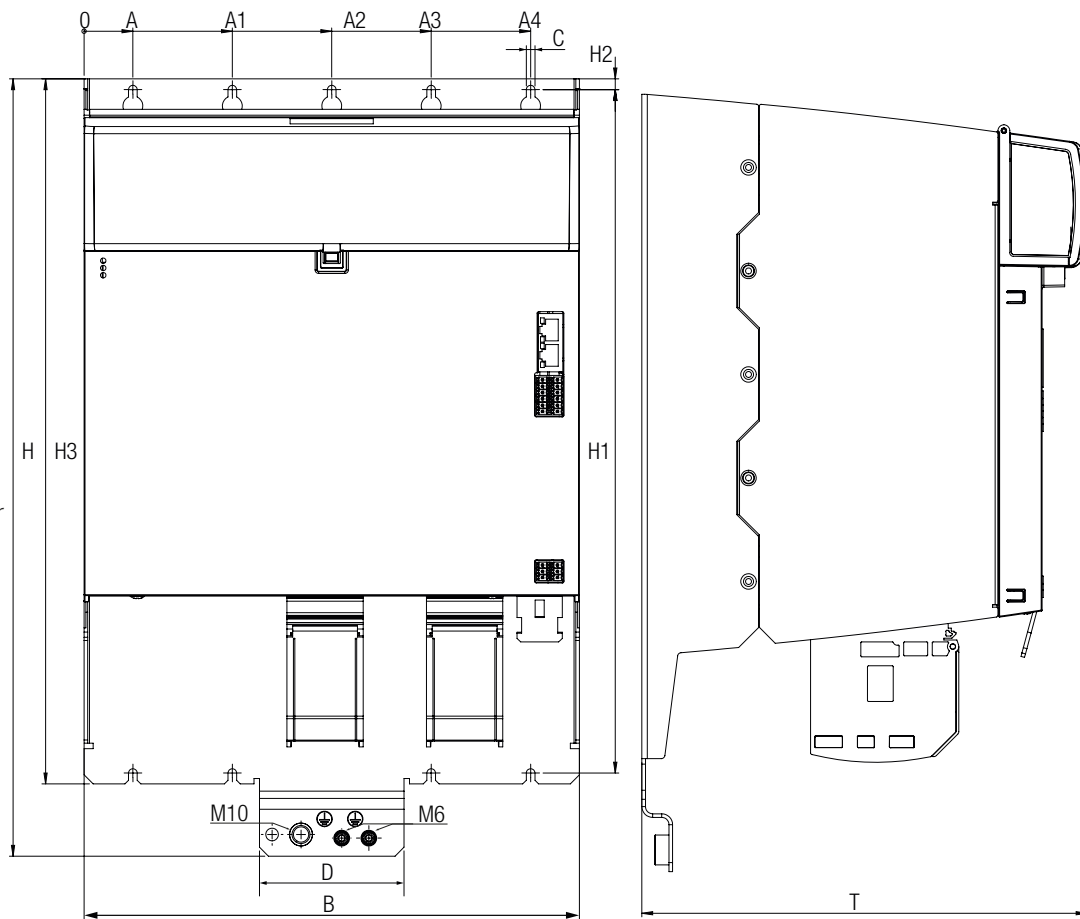
Figure 6.6 Dimensional sketches, KeDrive D3-EM energy manager
