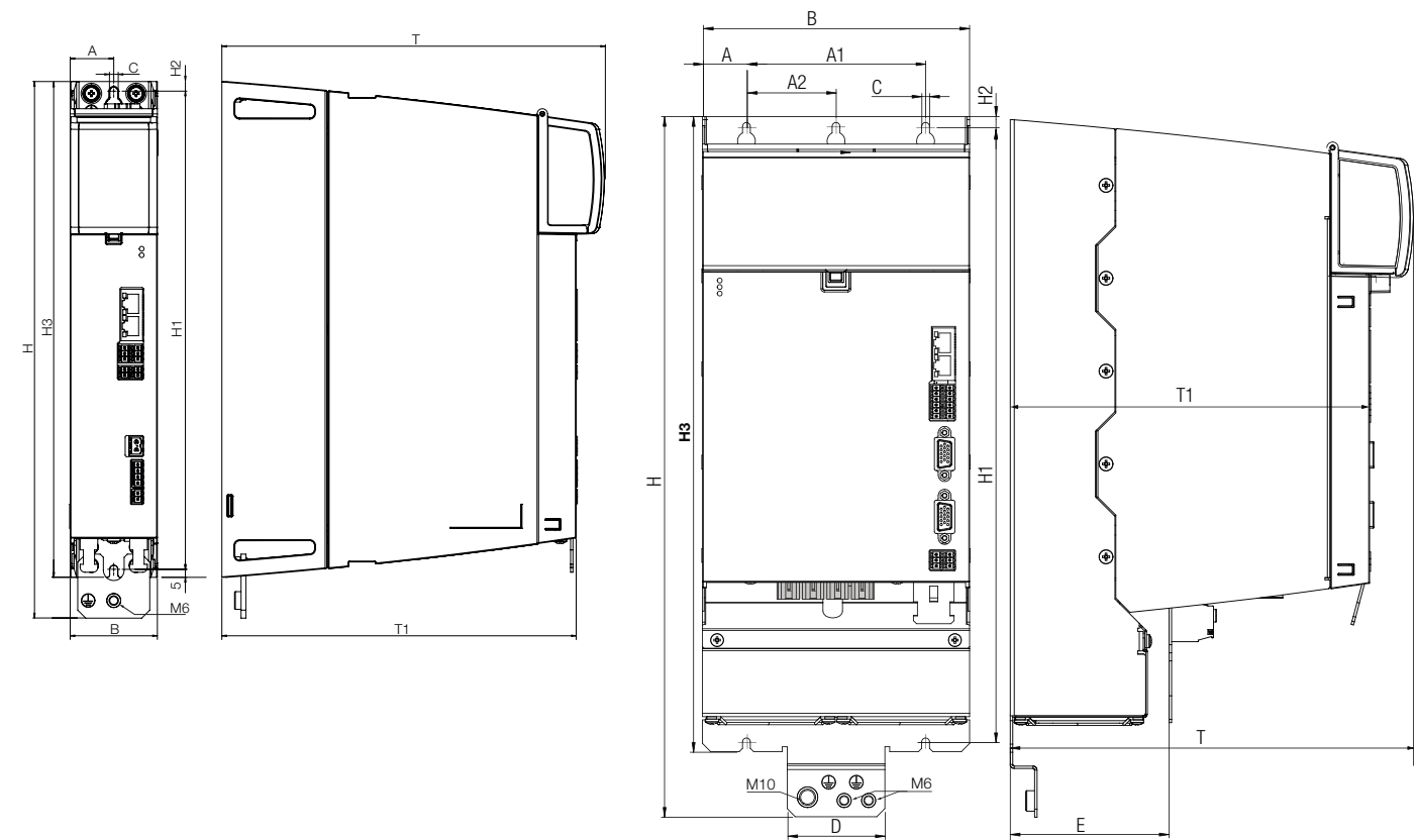
Figure 4.1 Dimensional sketches, KeDrive D3-DL 300 charging module Figure 4.2 Dimensional sketches, KeDrive D3-DP 310 supply module (heat sink)
