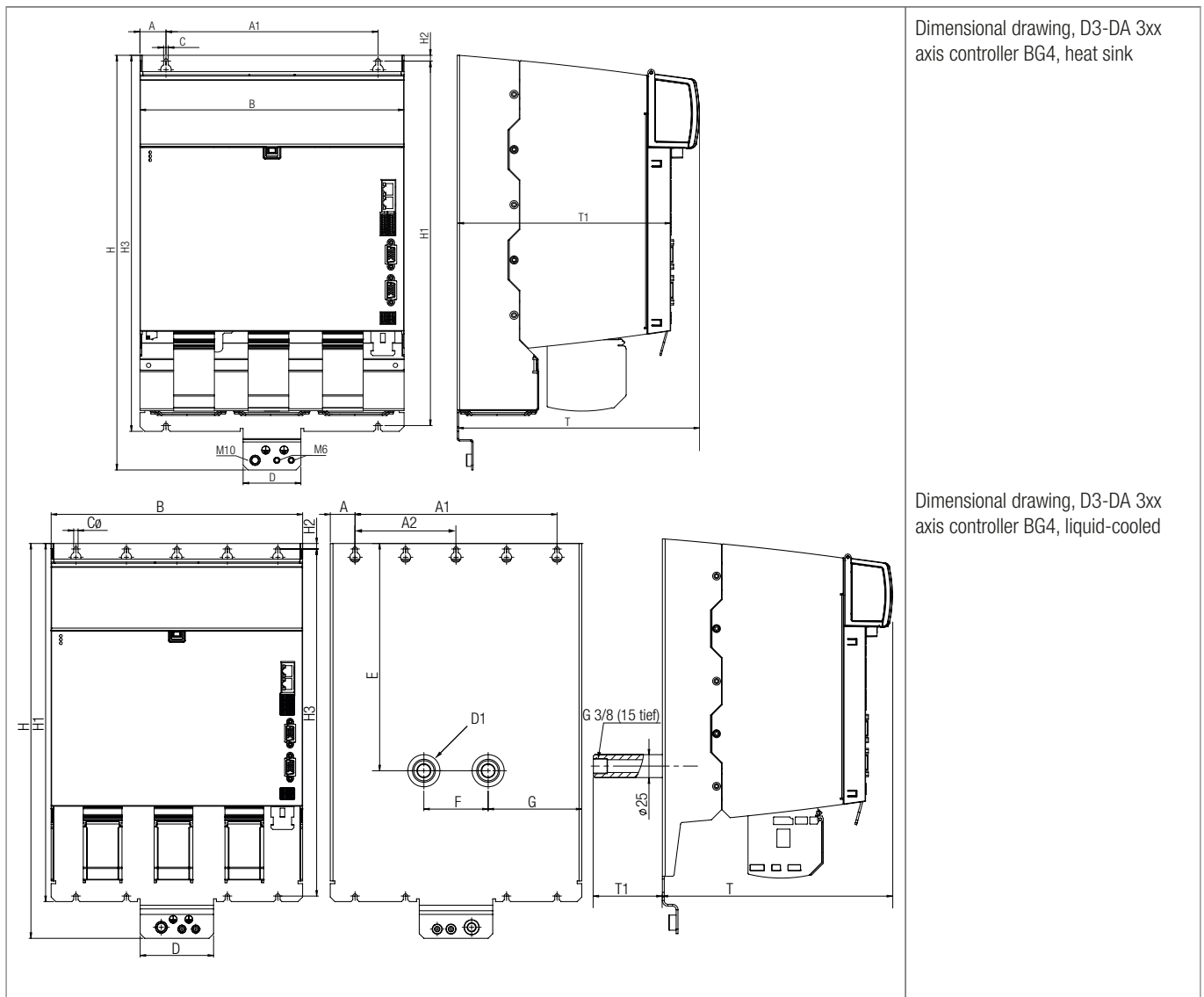
Figure 5.5 Dimensional drawings, KeDrive D3-DA BG4
