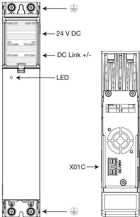
Figure 7.12 Connections, top
