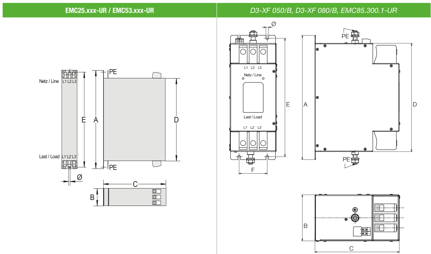
Figure 8.14 Dimensions
