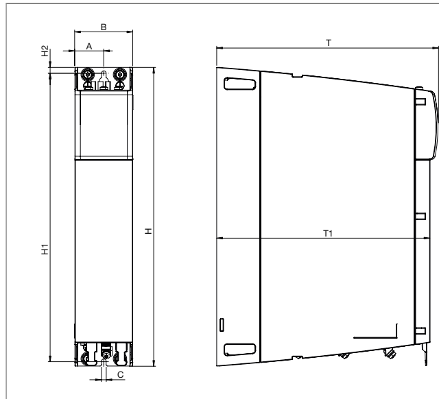
Dimensional sketch with heat sink (air-cooled) (BG1)
