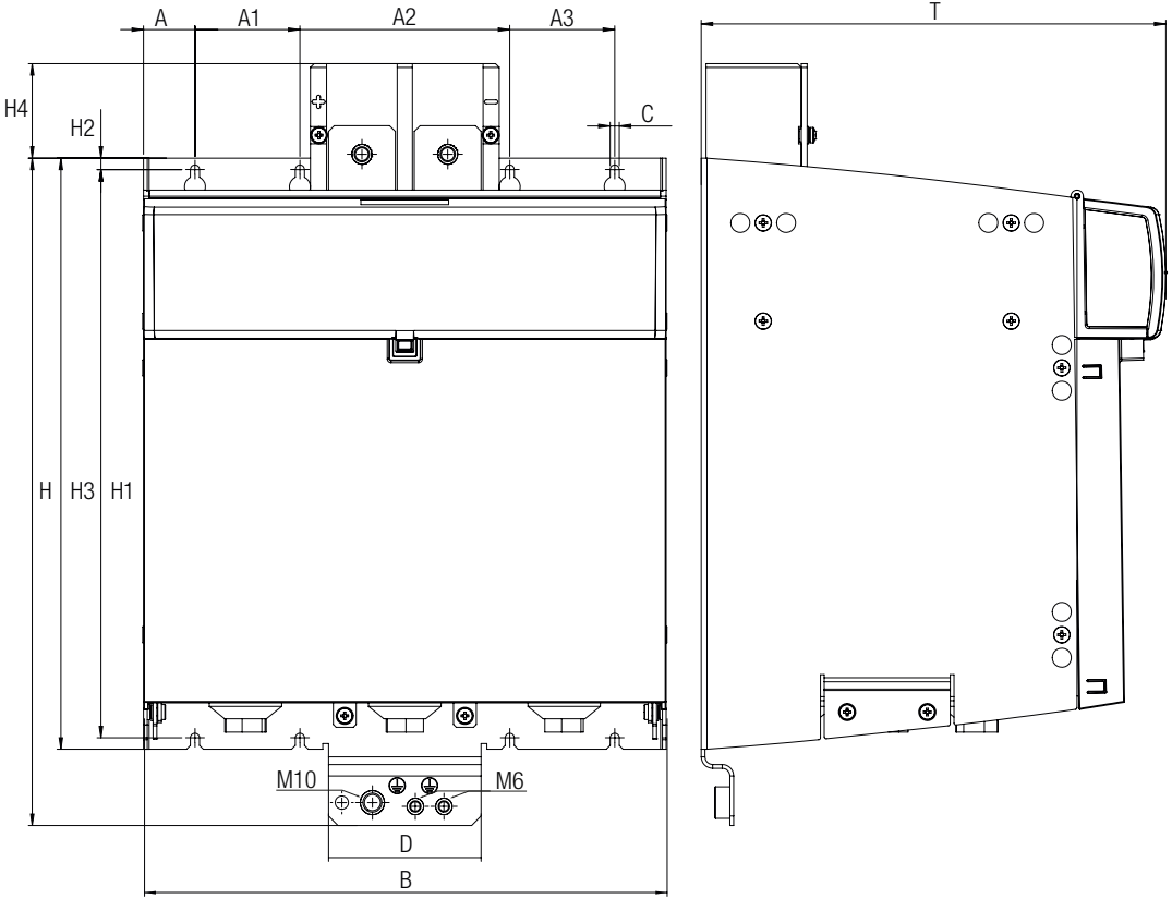
Figure 6.7 Dimensional sketches, KeDrive D3-ES energy storage device
