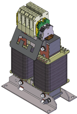
Figure 6.8 Choke module type D3-EL 120/A-0100-00
