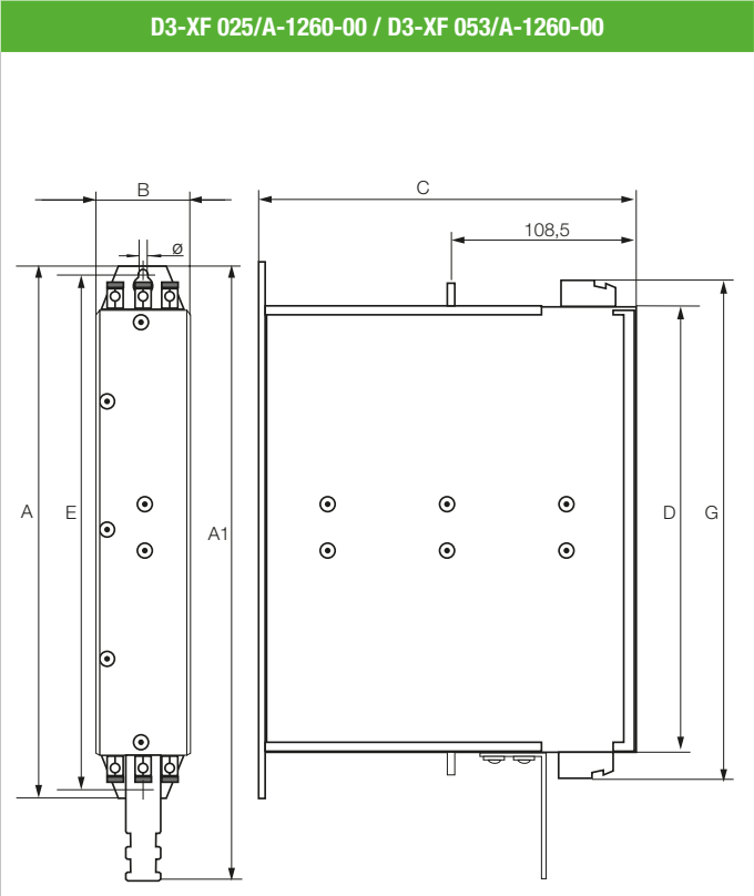
Figure 8.17 Dimensions
