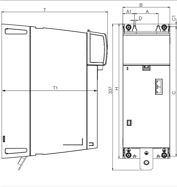
Figure 7.10 Dimensional drawing, D3-DC 300 module heat sink
