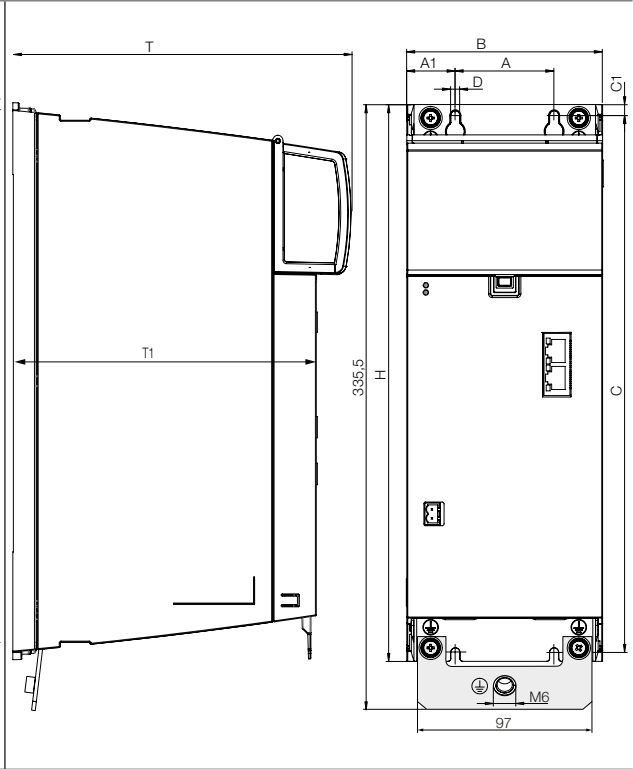
Figure 7.11 Dimensional drawing, D3-DC 300 module cold plate
