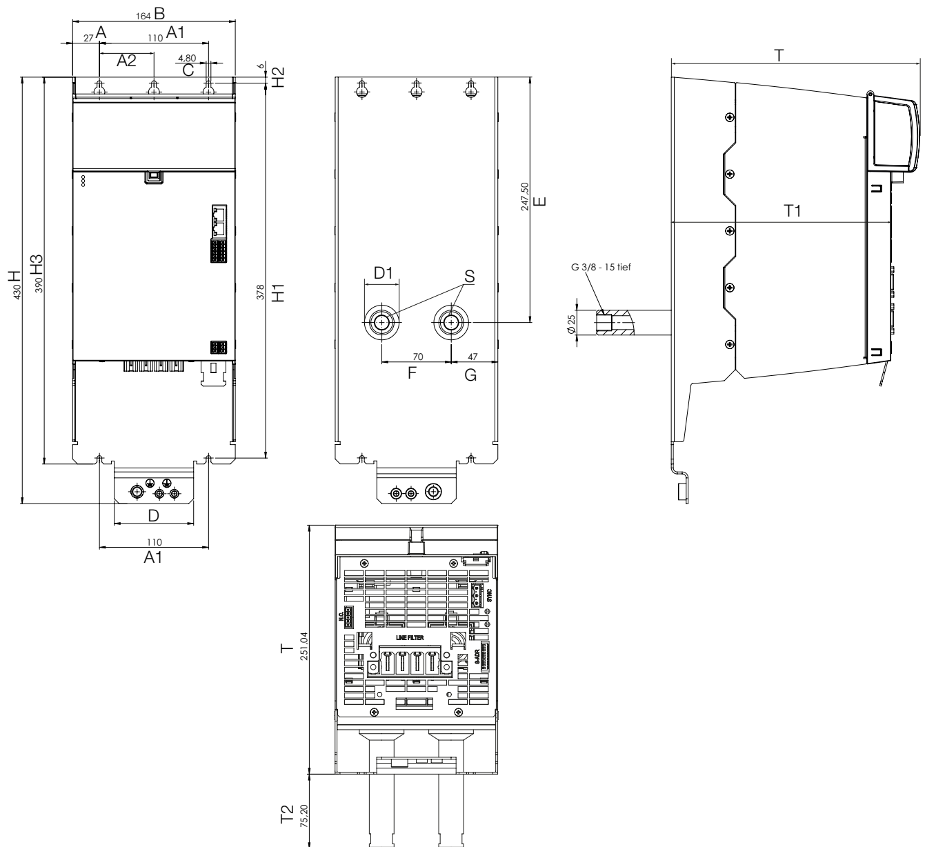
Figure 4.3 Dimensional sketches, KeDrive D3-DP 310 supply module, liquid cooling
