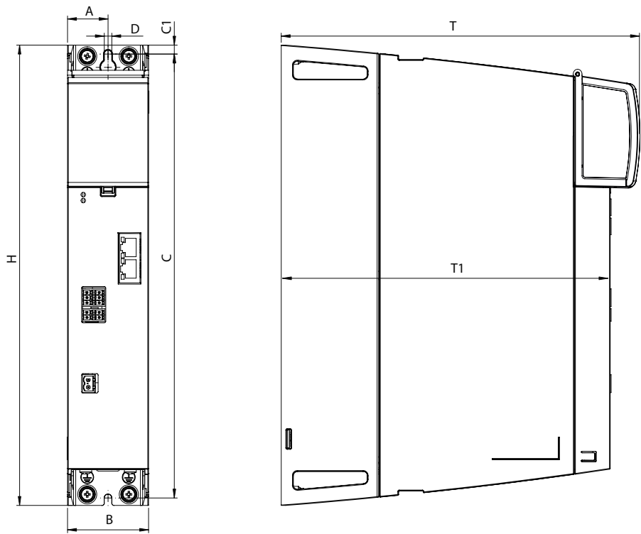
Figure 7.9 Dimensional drawing, D3-DE 300
