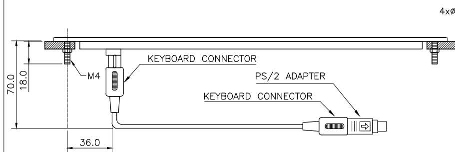
FLUSH PANEL SIDE VIEW BUILT-IN DEPTH
