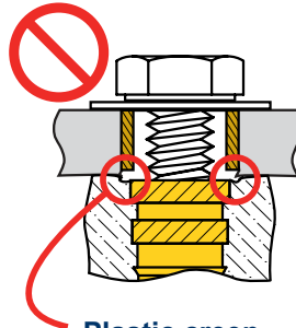
Plastic creep
