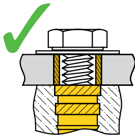
Proper configuration
