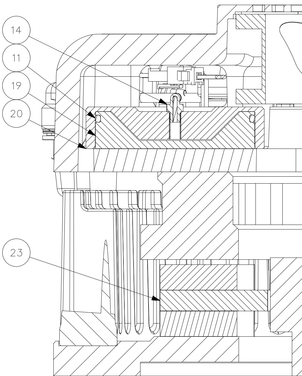
SECTION B—B
