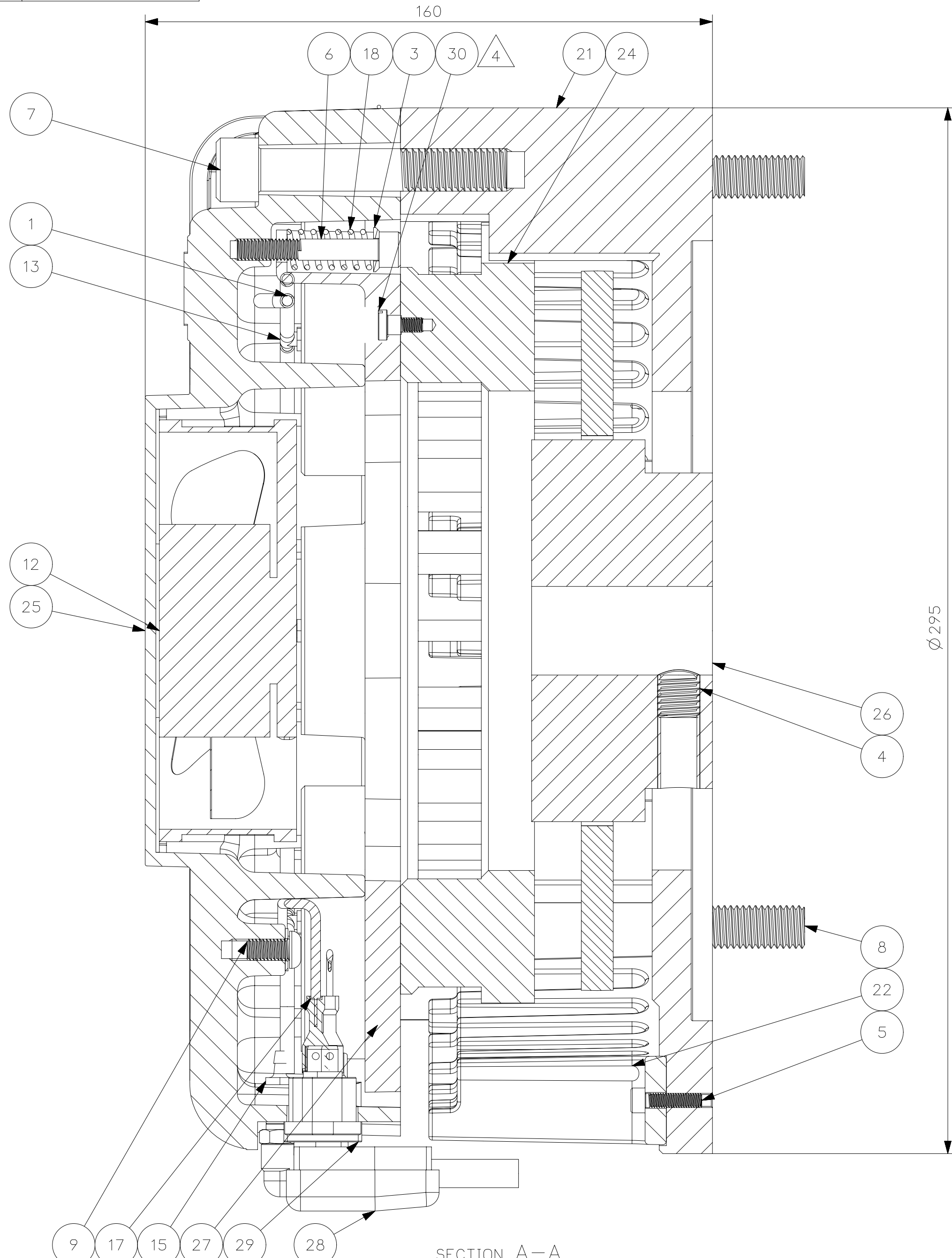
SECTION A—A
