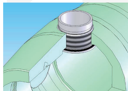
Seal seated against a flat surface
