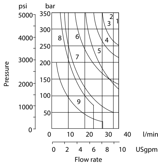
Graph 6 DC solenoid valves
