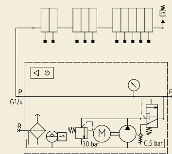
Hydraulikplan 2
