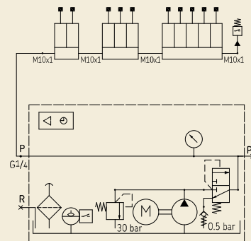
Hydraulikplan 1
