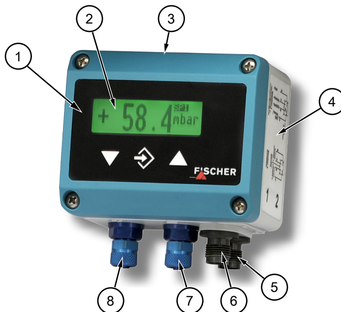
Illustration 1: Part designations
