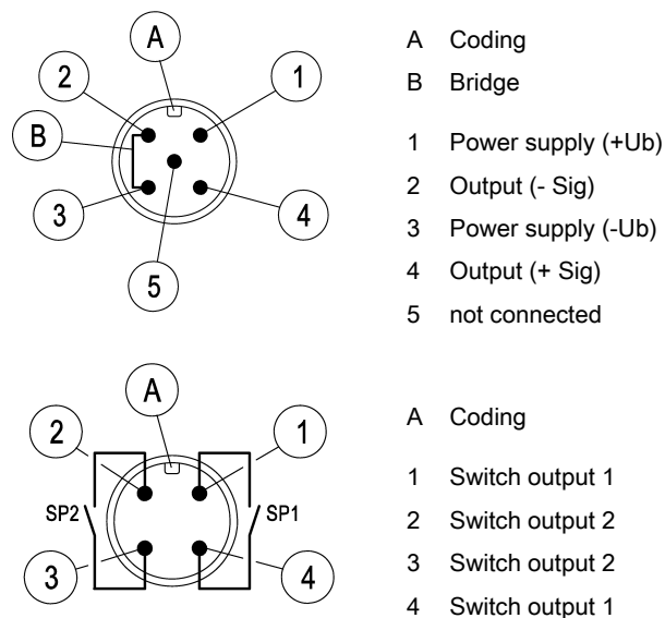
Illustration 3: Electrical connection DE45_LCD
