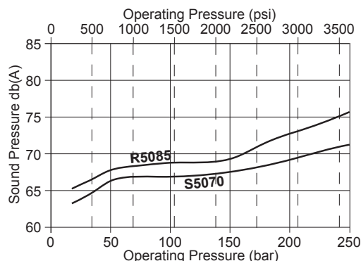
Q5 Sound Pressure at 1 metre - 2500 rpm
