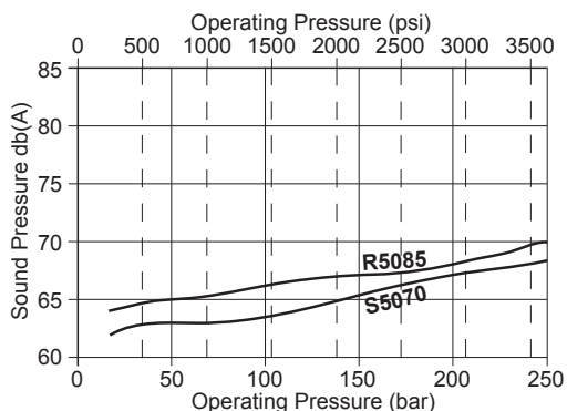
Q5 Sound Pressure at 1 metre - 1800 rpm
