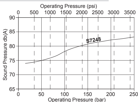
Q7 Sound Pressure at 1 metre - 1800 rpm
