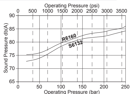
Q6 Sound Pressure at 1 metre - 2400 rpm
