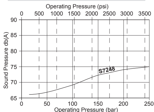
Q7 Sound Pressure at 1 metre - 1500 rpm
