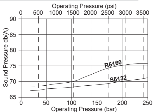
Q6 Sound Pressure at 1 metre - 1800 rpm
