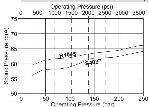
Q4 Sound Pressure at 1 metre - 2500 rpm
