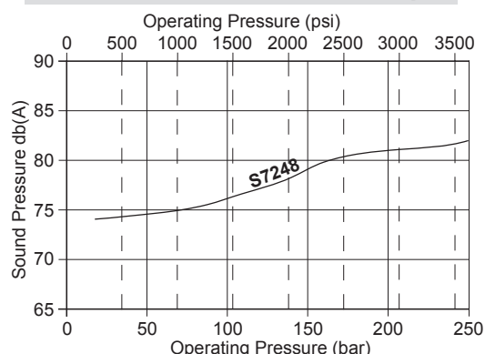
Q7 Sound Pressure at 1 metre - 2250 rpm
