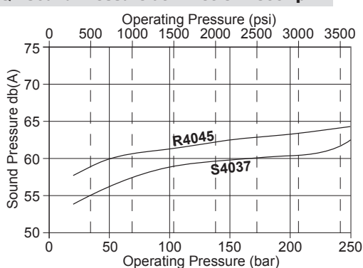
Q4 Sound Pressure at 1 metre - 1800 rpm
