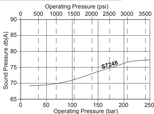
Q7 Sound Pressure at 1 metre - 1000 rpm
