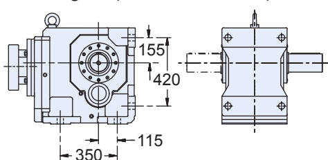
Size K10 Mounting Feet (Dimensions b3 and b4)
