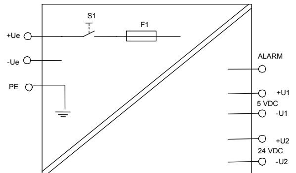
Figure 1: Block diagram 560PSU01
