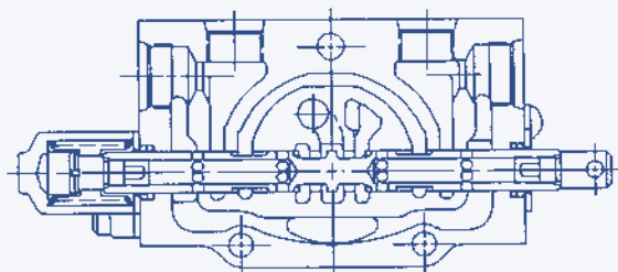
FULL SECTION VIEW OF P/N: 5002E36
