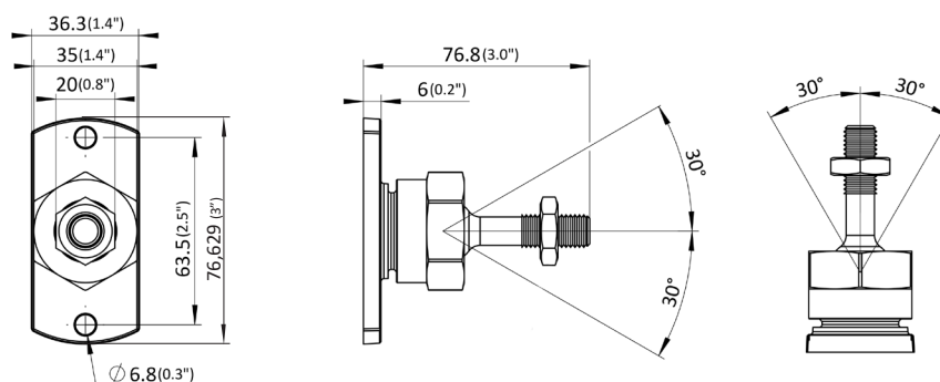
Figure 1 Dimension- and assembly drawing for art. 20856
