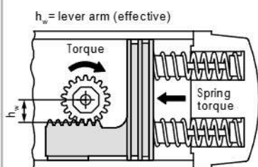
Fig. SC05: Top view of a single acting actuator
