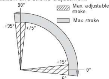
Rotation and stroke adjustment
