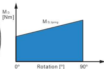
Diagram SC06: Principle of the spring torque
