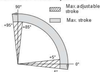
Rotation and stroke adjustment
