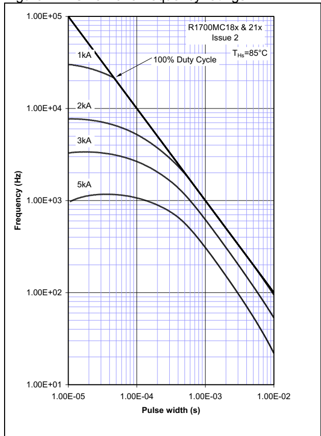
Figure 12 - Sine wave frequency ratings
