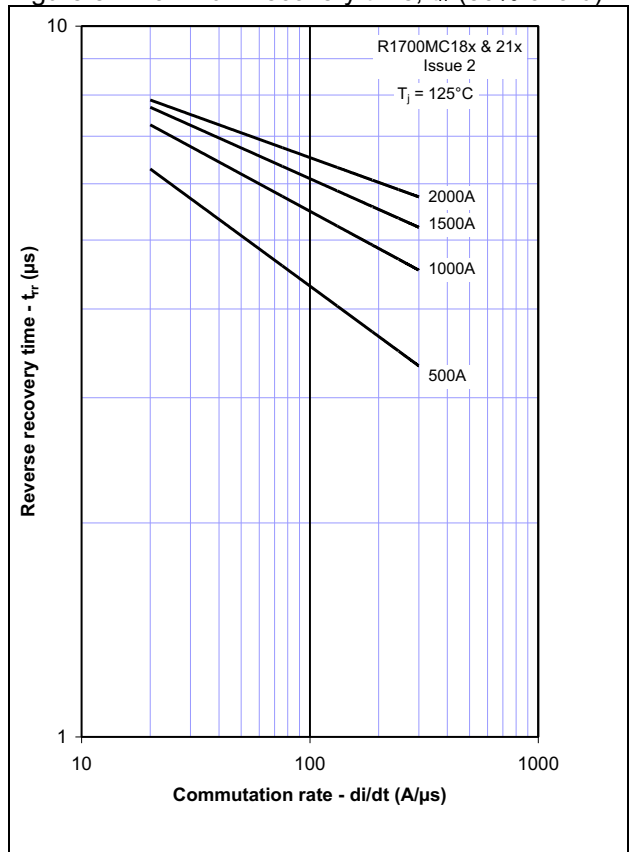
Figure 8 - Maximum recovery time, t_{rr} (50% chord)
