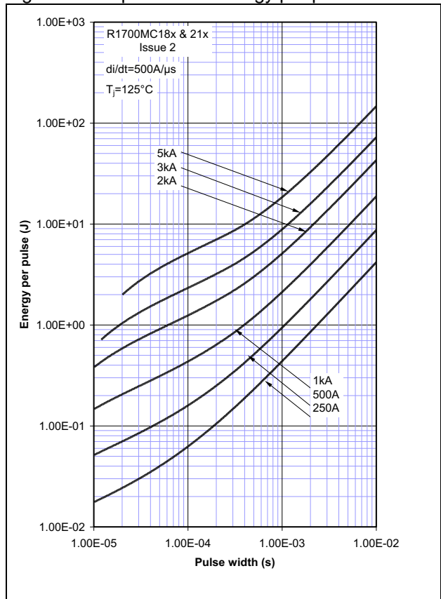
Figure 18 - Square wave energy per pulse
